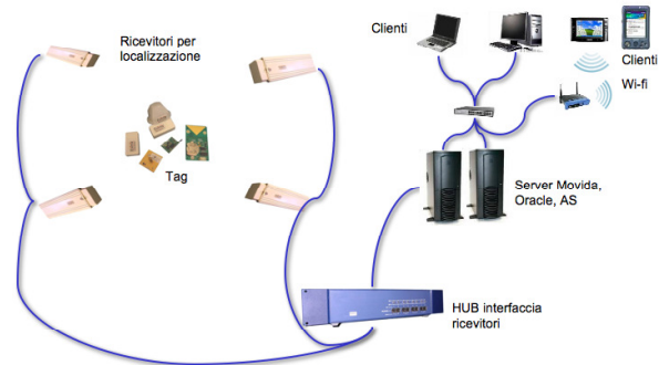
The diagram shows the typical configuration in HA of an E_RTL system, usable through various client applications
